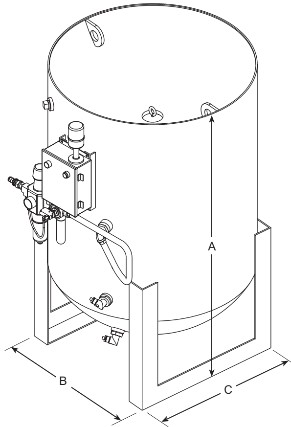
Dense Phase Hopper Dimensions and Weight
